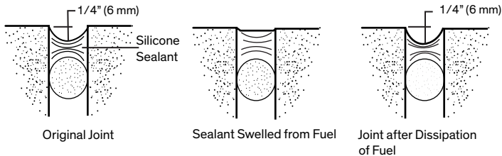
Figure 2. Effect of Fuel Spill on DOWSIL™ Silicone Joint Sealant
