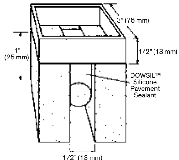
Figure 1. Simulated Fuel Spill Test Joint
