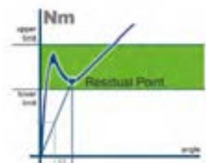
Residual Torque (VDI-VDE 2645-3)
