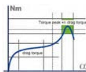
Prevailing torque automatic compensation
