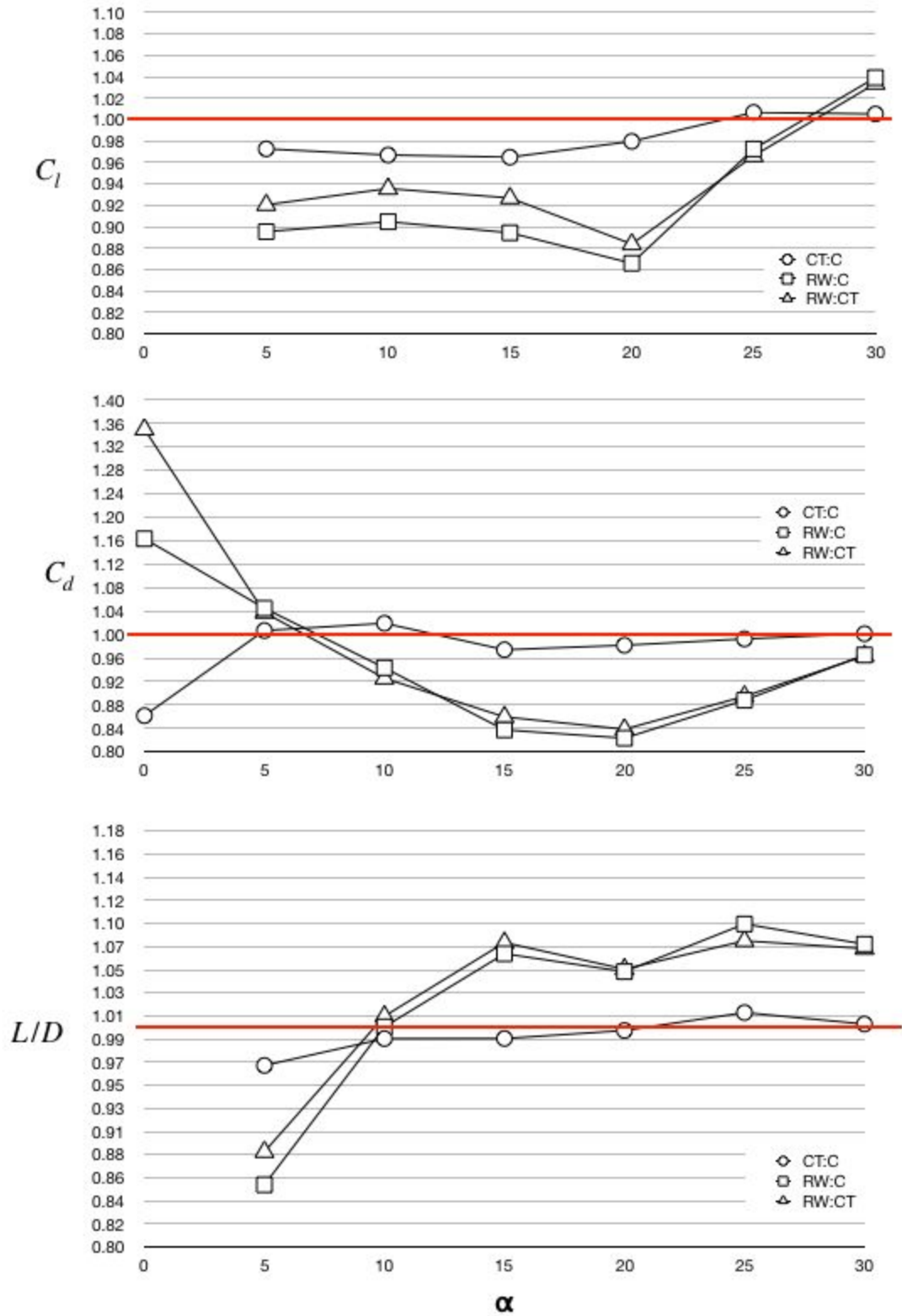
Figure S1. Relative comparisons of data in Figure 3. For RW, C_l improves after 25°, but notice increasing trend begins at 20°. Reduced C_d begins after 5° and improved L/D at 10°.
