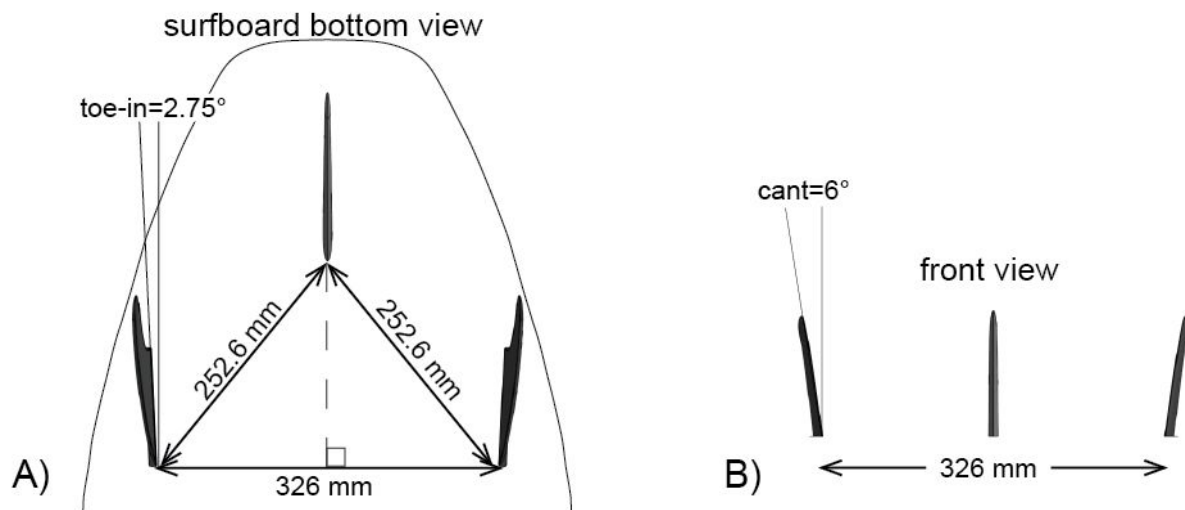
Figure S2. Thruster fin positioning used in simulations. Toe-in refers to the angle the thruster fins are angled towards the nose. Cant refers to the angle the thruster fins are tilted outwards, towards the rail or edge of the surfboard. Cant and toe-in are symmetrical for both thruster fins.
