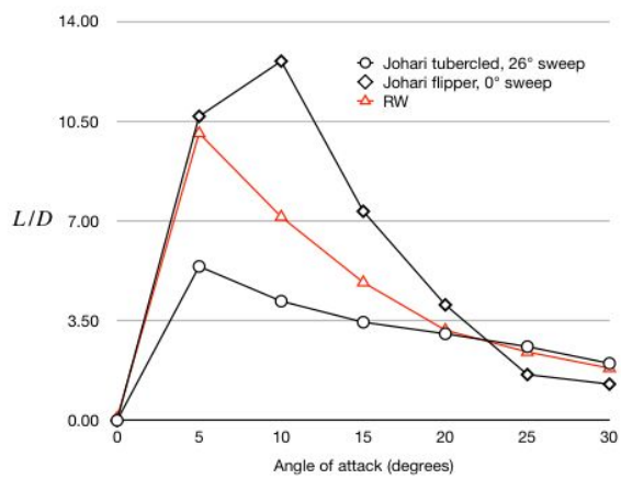
Figure S2. Comparisons of RW to Johari [6] flipper design at 0° sweep and similar aspect ratio, and a swept design with lower aspect ratio. Flows near Re \approx 2.7-2.8 \times 10^5 .
