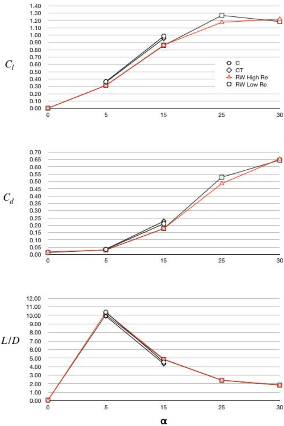
Figure S3. High Re ( 1.8 \times 10^6 ) results. Only 5 and 15° \alpha tested for C and CT.
