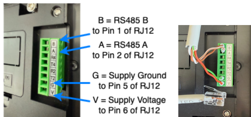
Figure 10. Pin assignments for connection from screen to RJ12
