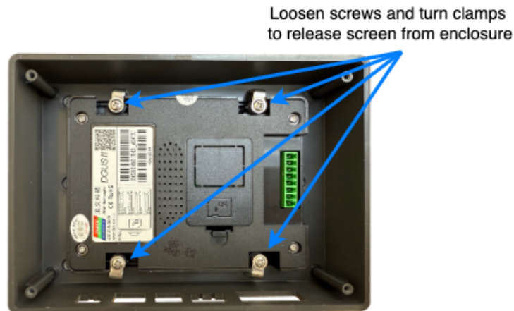
Figure 8. Loosen screws holding screen to enclosure
