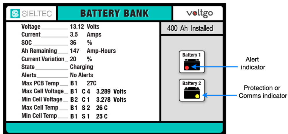
Figure 17. Alert and Protection or Comms indicators
