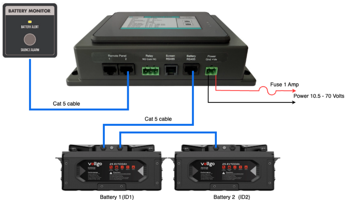
Figure 3. Basic cabling configuration
