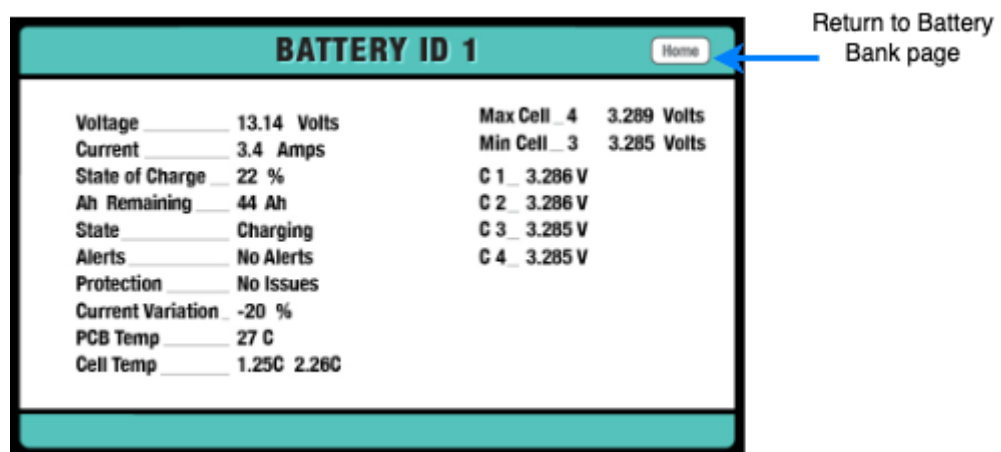
Figure 14. Individual battery page
