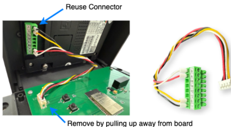
Figure 7. Remove existing screen connection
