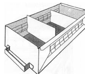
8104 Box of 100 Steel Partitions Partition Size: 5-1/8"Wx2-7/8"D Fits Drawer Size: 2-3/4"Hx5-3/8"Wx11-1/2"D Ship Weight 5 lbs.
