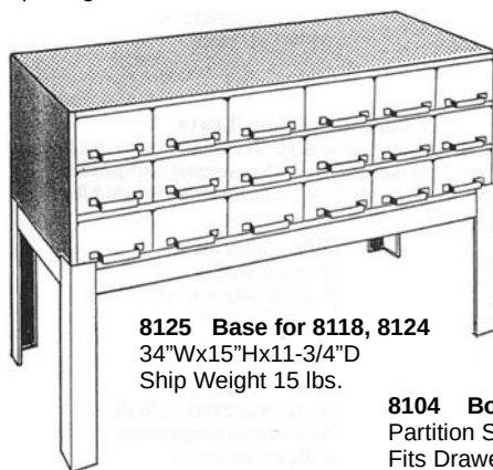
8118 18 Drawer Cabinet 35"Wx10-3/4"Hx11-1/2"D Drawer Size: 2-3/4"Hx5-3/8"Wx11-1/4"D Partitions: Includes 36 Ship Weight 50 lbs.
