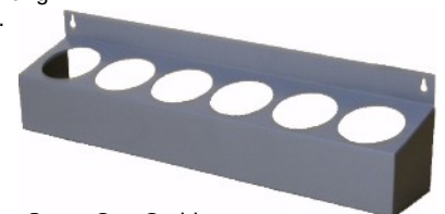
9006 Spray Can Caddy 21"Wx5-3/8"Hx3-7/8"D Compartment Back 3-15/16"H Front 2-15/16"H Hole size 3" diameter Keyholes for mounting Ship Weight 4 lbs.
