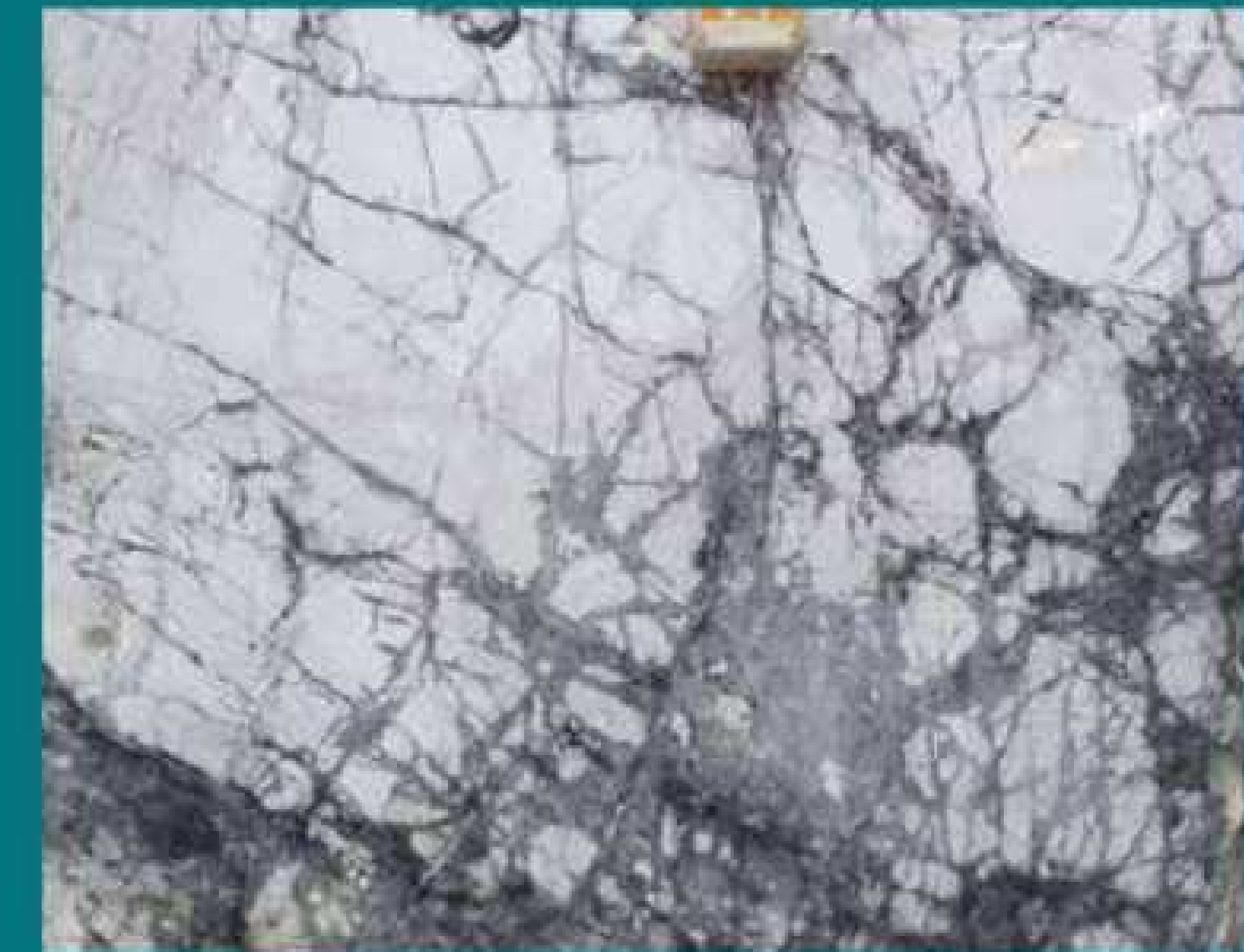
ICEBERG - TURKEY
