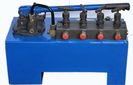
GANG JACKING HAND PUMP WITH INDEPENDENT NEEDLE VALVES
