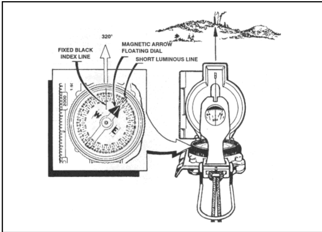
Figure 9-4. Compass preset at 320^\circ degrees.
