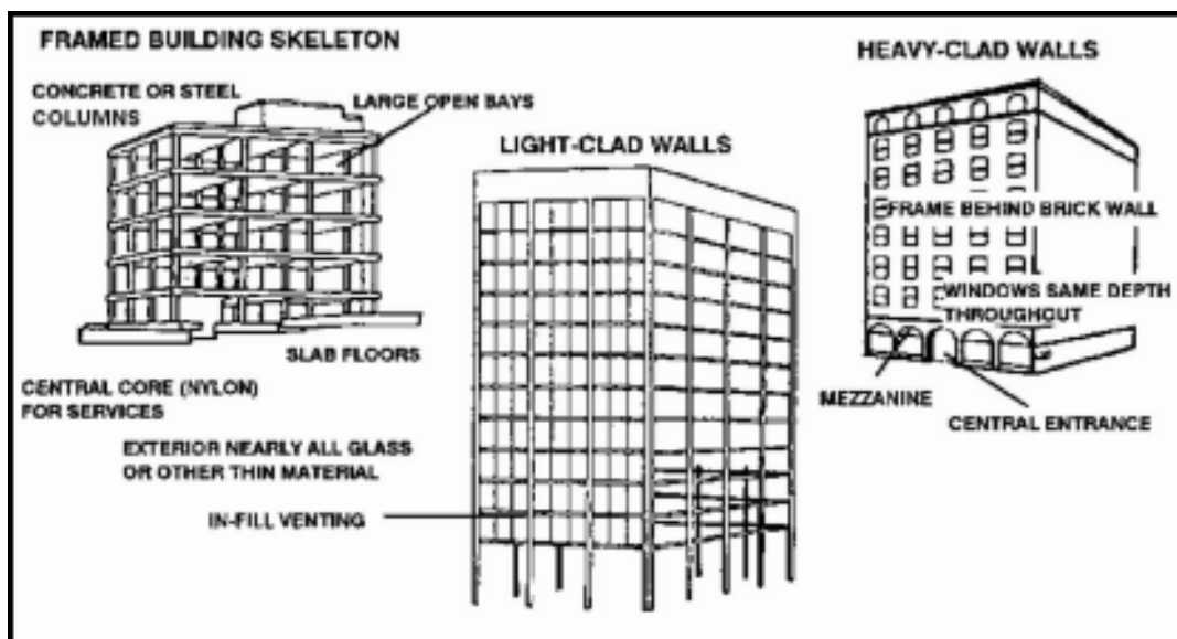
Figure 2-22. Framed buildings.
