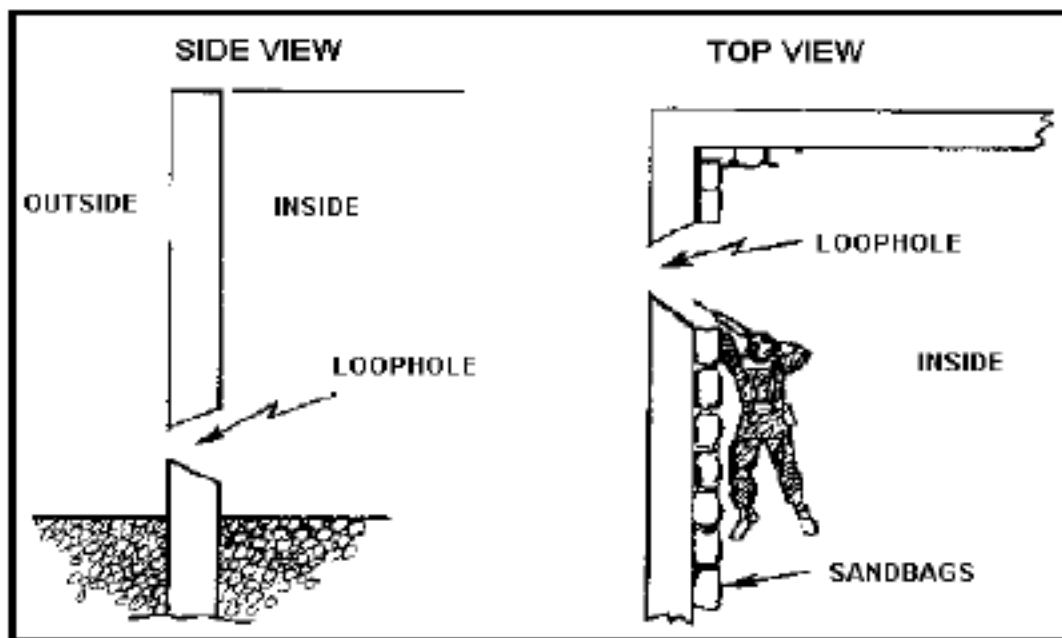
Figure 3-48. Prepared loophole.
