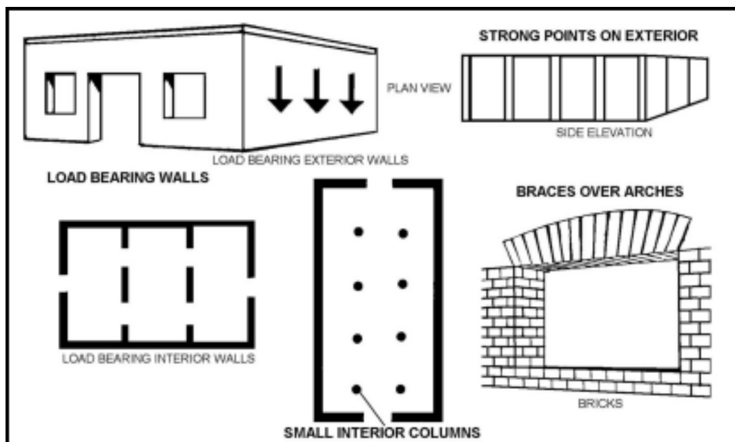
Figure 2-16. Mass-construction buildings.
