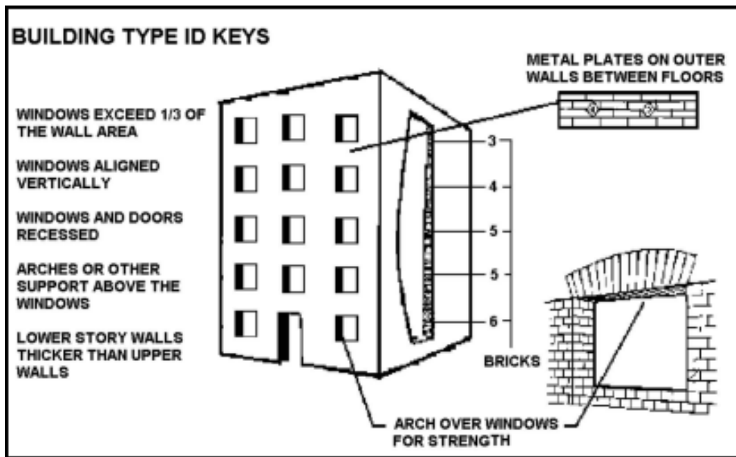
Figure 2-17. Brick buildings.
