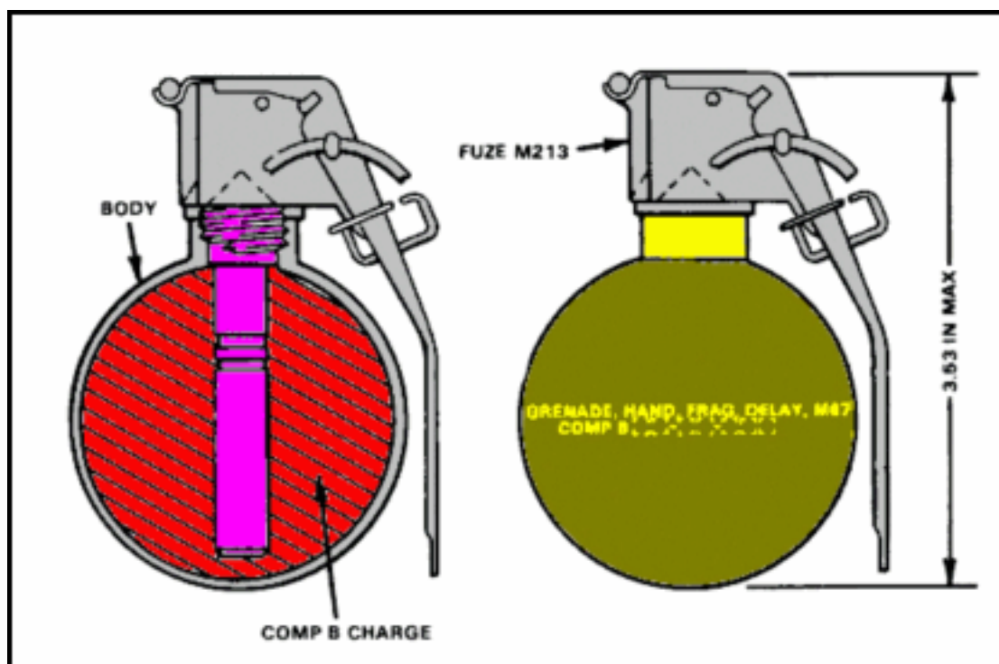
Figure 3-21. Fragmentation grenade.
