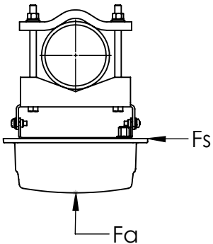
WIND LOADING
