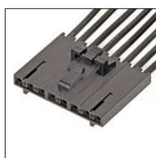
SL (Positive Latch) 2.54mm Pitch
