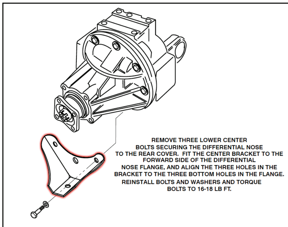
Figure 3 - Center Bracket Installation to Differential
