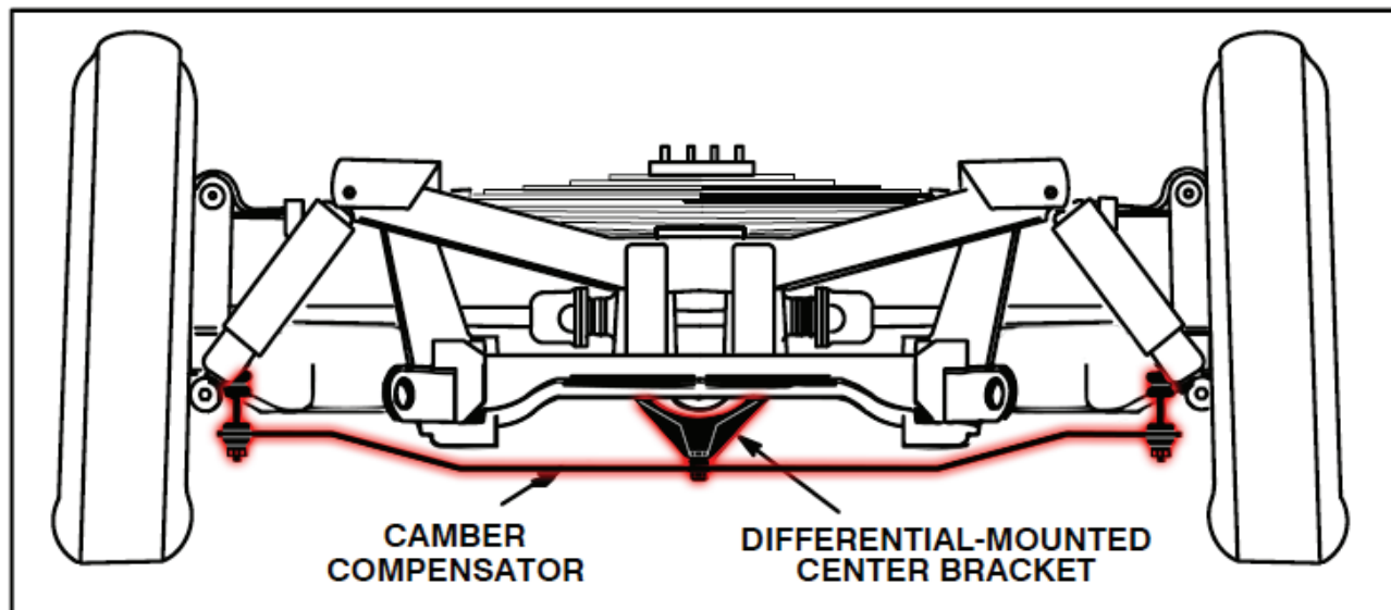
Figure 2 - Camber Compensator (Rear Elevation)
