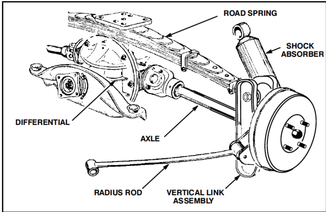
Figure 1 - Suspension Layout before Installation (Forward of Left Side Shown)
