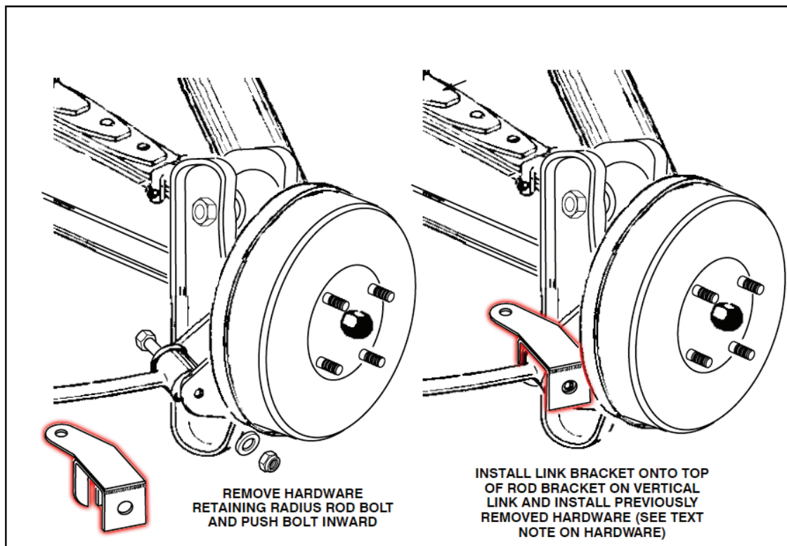
Figure 4 - Outer Link Side Bracket Installation (Left side shown)
