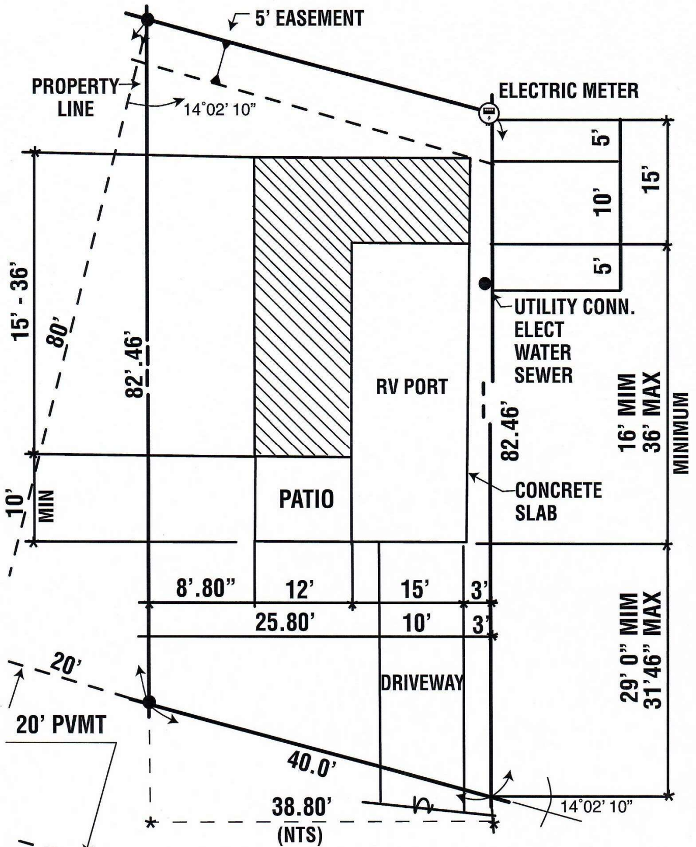
PLOT PLAN 1" = 10' TAHI - 1
