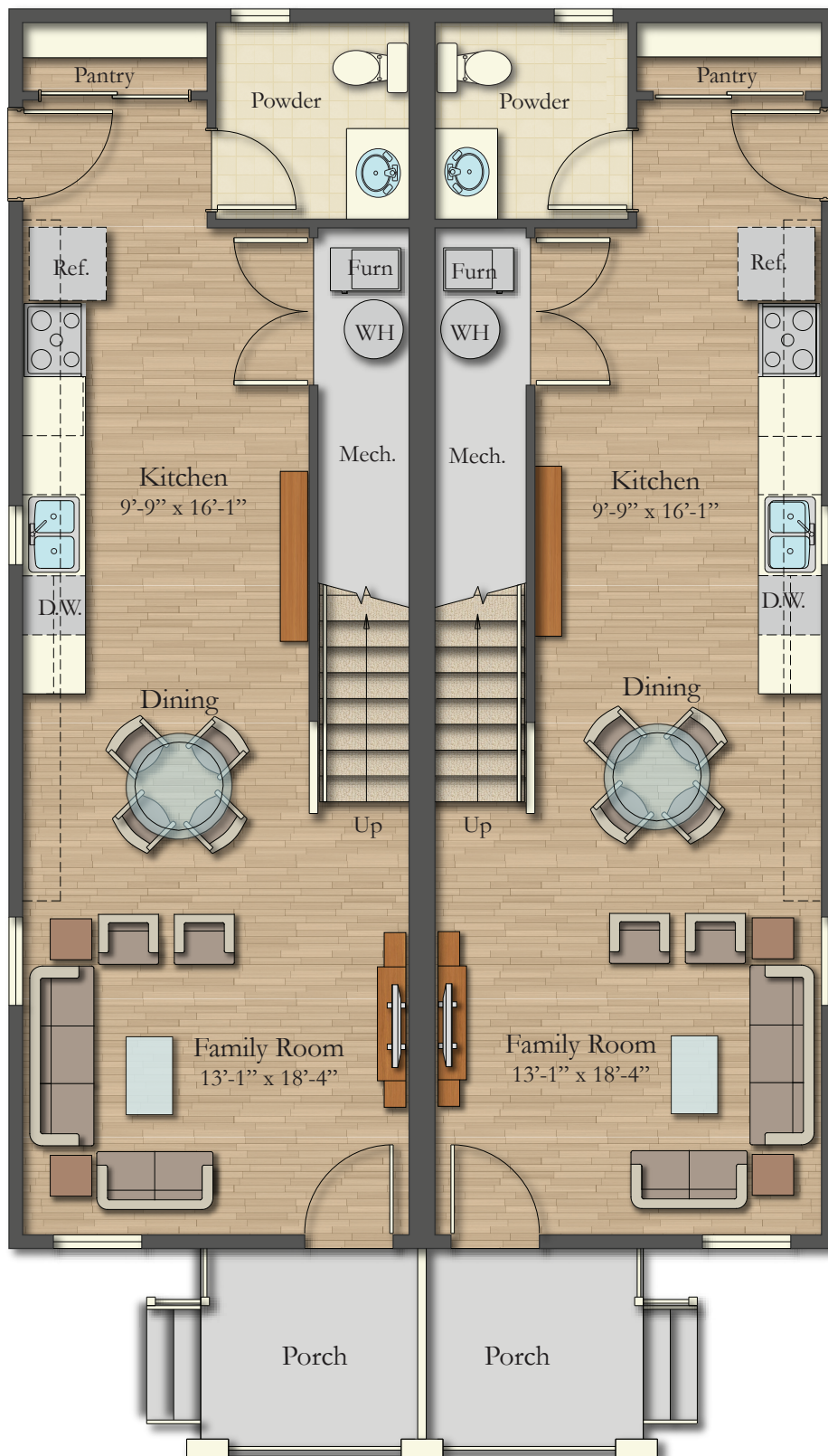
Main Floor
