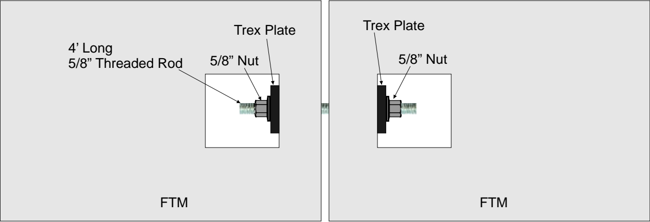
FTM Connection Detail
