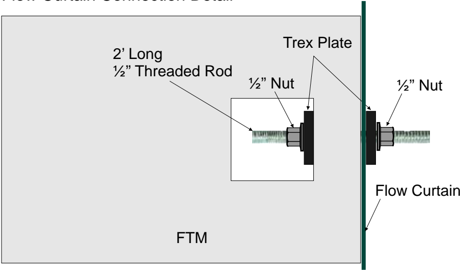
Flow Curtain Connection Detail
