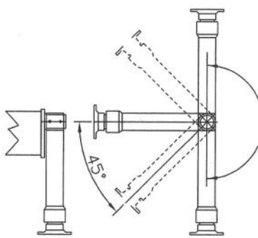
Tilt-up Leg
