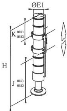
Adjustable Leg
