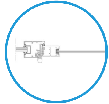
Head track horizontal Alu frame single glass
