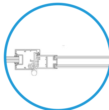
Head track horizontal Alu frame double glass
