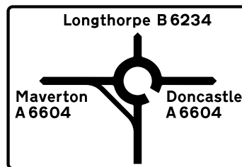
Segregated left-turn lane
