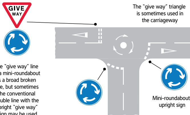
Typical mini-roundabout junction
