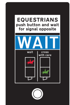
Push-button unit for far-side signals
