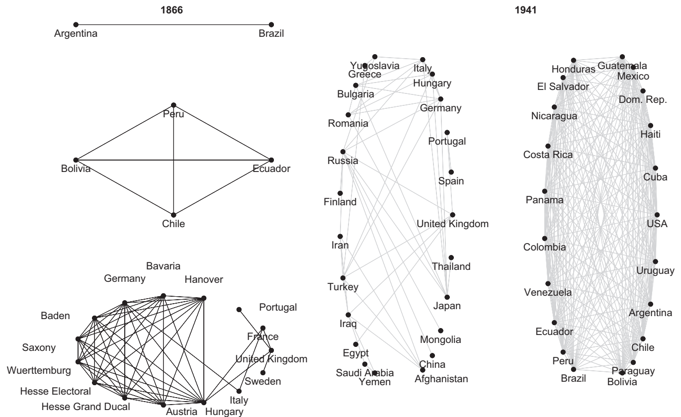
Fig. 1. Two of the alliance graphs, 1866 and 1941. The 1941 graph consists of two components: a complete graph on 21 vertices (the US and its Latin American allies) and a sparse graph on 23 vertices with 45 edges, corresponding to Europe and Asia.
