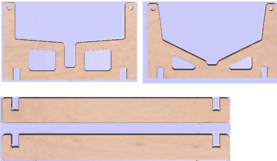
12mm Stand (4 pieces)
