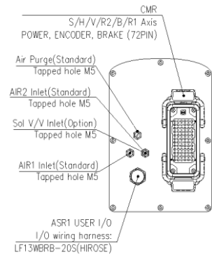
View C: Application cable connection part
