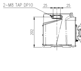
View G: Application part mounting
