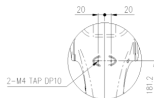
View E: Application part mounting detail
