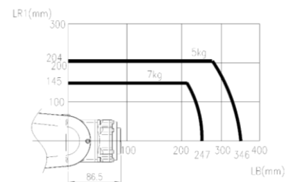
Wrist-axis torque line diagram
