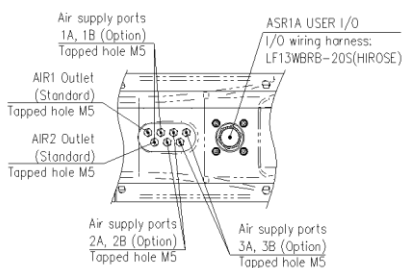
View D: Application cable connection part
