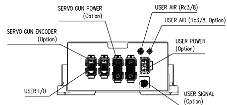
View D: Application cable connection part (Option)
