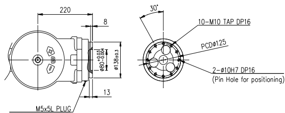
View A: Detailed drawing of the wrist attachment part
