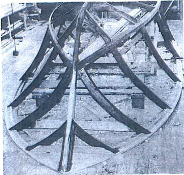
HULLS UNDER CONSTRUCTION
