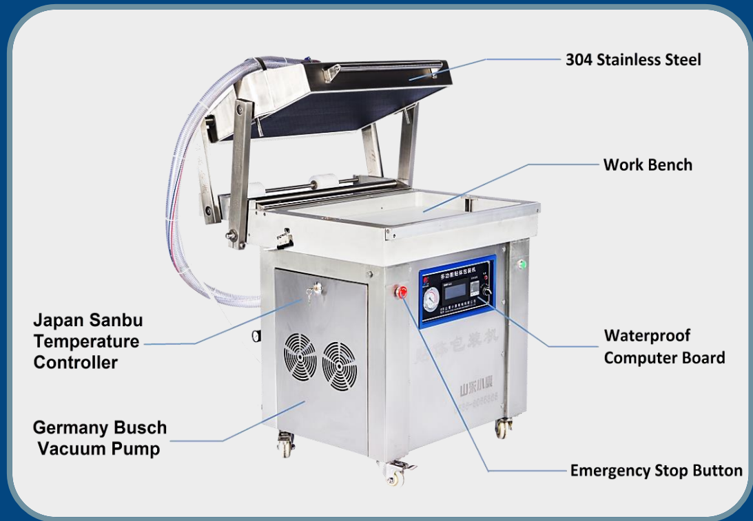
SKIN VACUUM PACKING MACHINE
