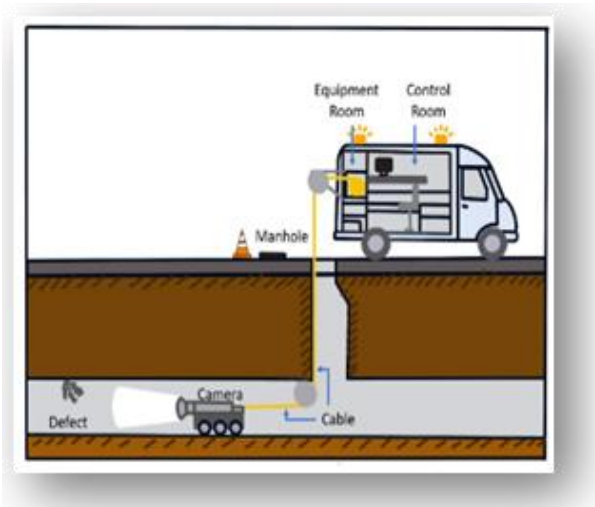
Figure 1. Sewer CCTV Inspection
