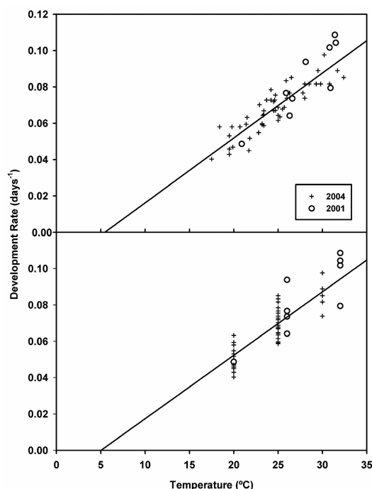
Fig. 3. Linear regression of transformed ( \text{days}^{-1} ) developmental time from egg to adult P. regina by using rearing-container (A) and set-chamber (B) temperatures. A = 0.0036x - 0.0195 , R^2 = 0.79 ; and B = 0.0035x - 0.0175 , R^2 = 0.74 . For x-intercept, A = 5.4^\circ\text{C} and B = 5.0^\circ\text{C} .
