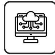
Web Services
