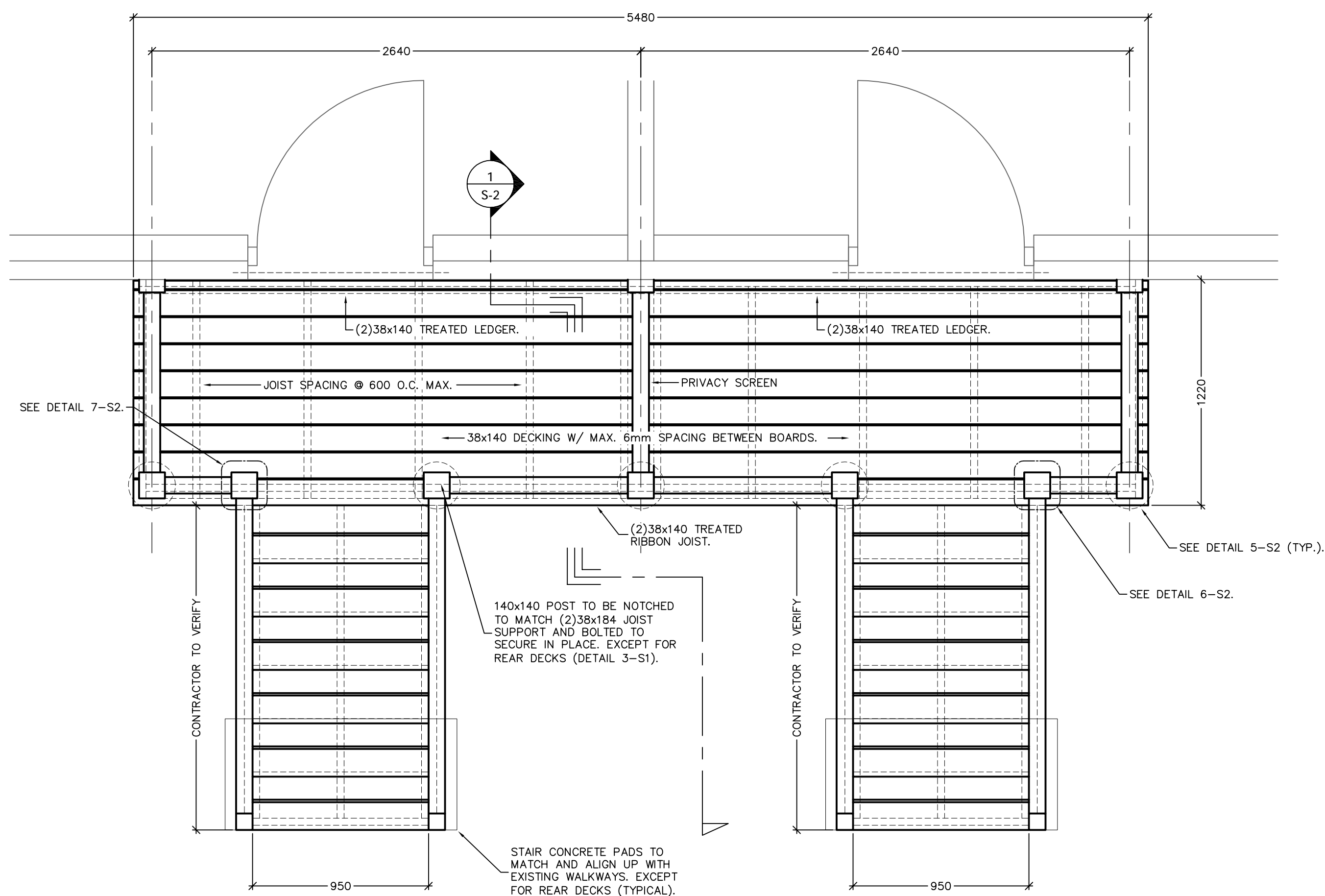
2 DECK PLAN (FRONT) - DECK STYLE #3 SCALE: 1:20
