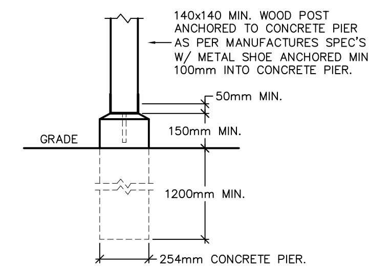
5 TYPICAL PIER DETAIL SCALE: NTS
