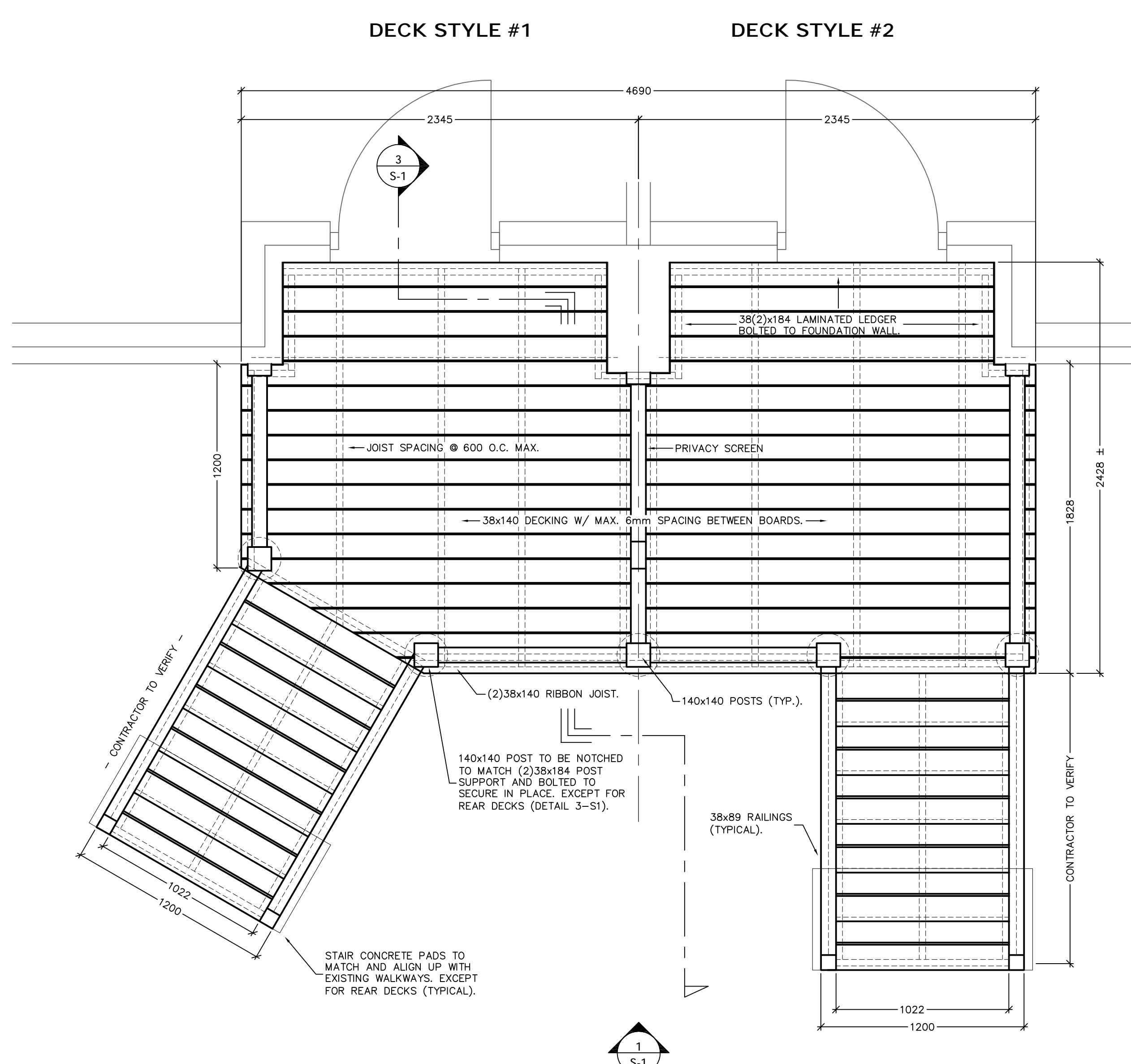
2 DECK PLAN - STYLE #1 AND #2 SCALE: 1:20
