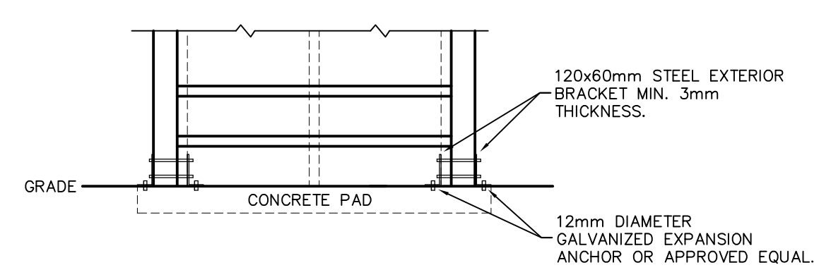
5 FRONT VIEW STRINGER SCALE: NTS
