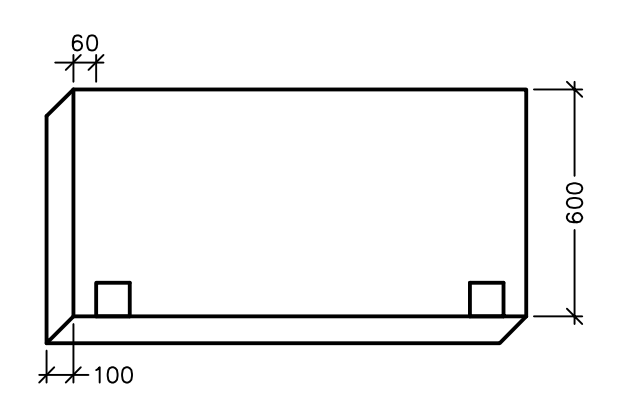
4 TYPICAL CONCRETE PAD DETAIL SCALE: NTS
