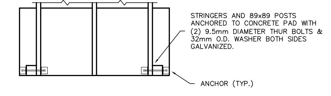
6 PLAN VIEW STRINGER SCALE: NTS
