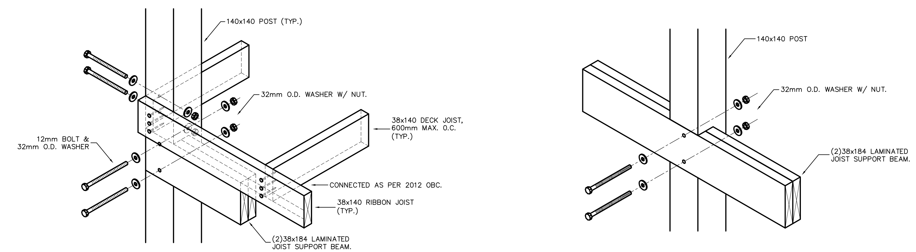
7 DECK FASTENING DETAILS - (EXCEPT REAR DECKS) SCALE: NTS
