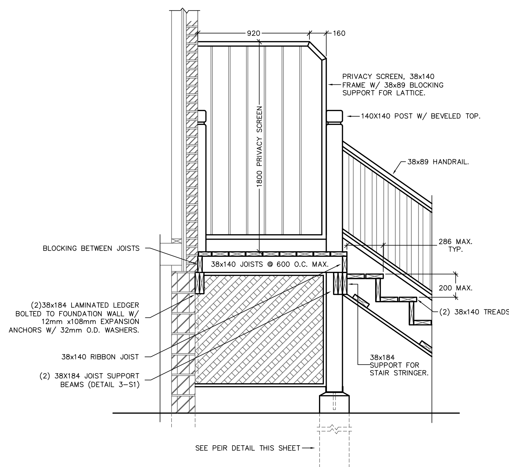
1 SECTION - DECK STYLE #3 SCALE: 1:20
