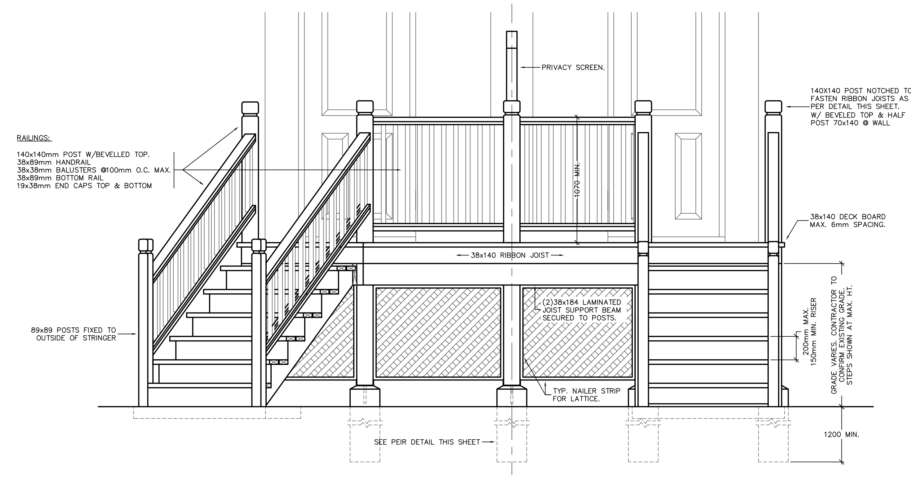
1 TYPICAL ELEVATION - DECK STYLE #1 AND #2 SCALE: 1:20
