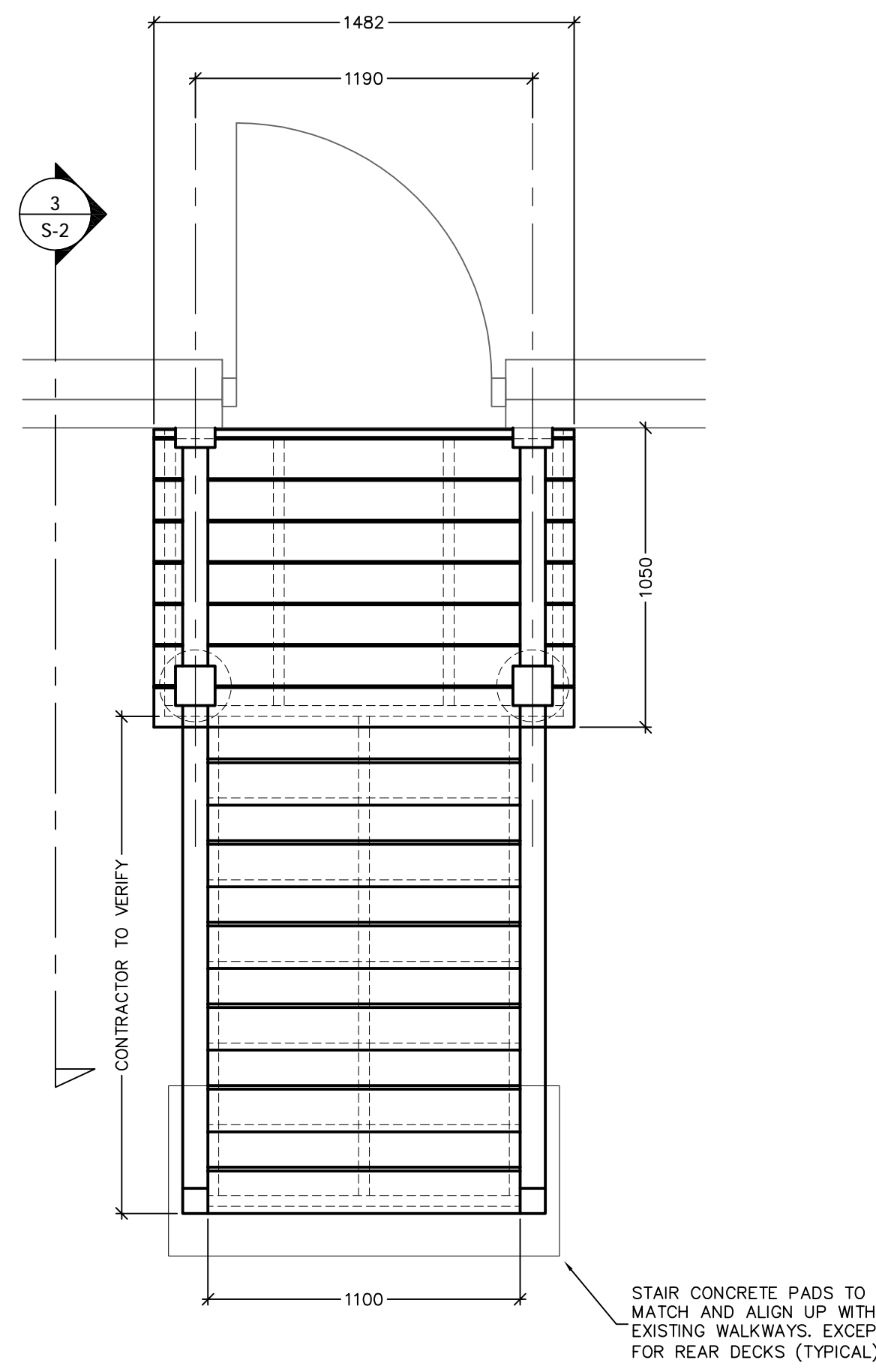
4 DECK PLAN (REAR) - DECK STYLE #4 SCALE: 1:20
