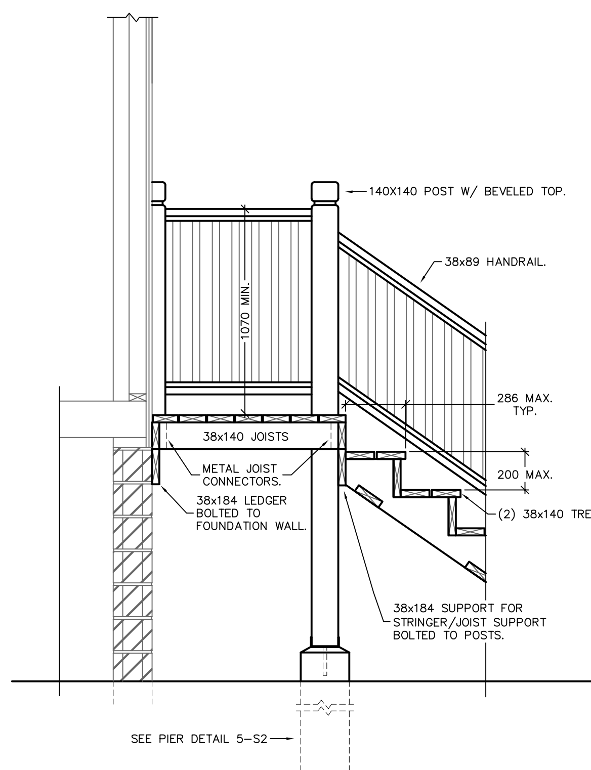
3 SECTION - DECK STYLE #4 SCALE: 1:20
