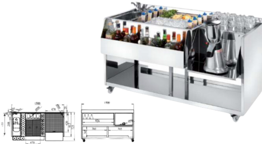
MODC001 SUPER COMPACT Cocktail Station St. Steel 18/10 150x70x83h cm
