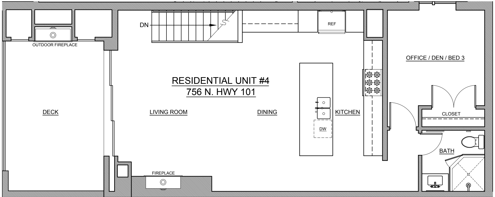
RESIDENCE #4: SECOND FLOOR PLAN
