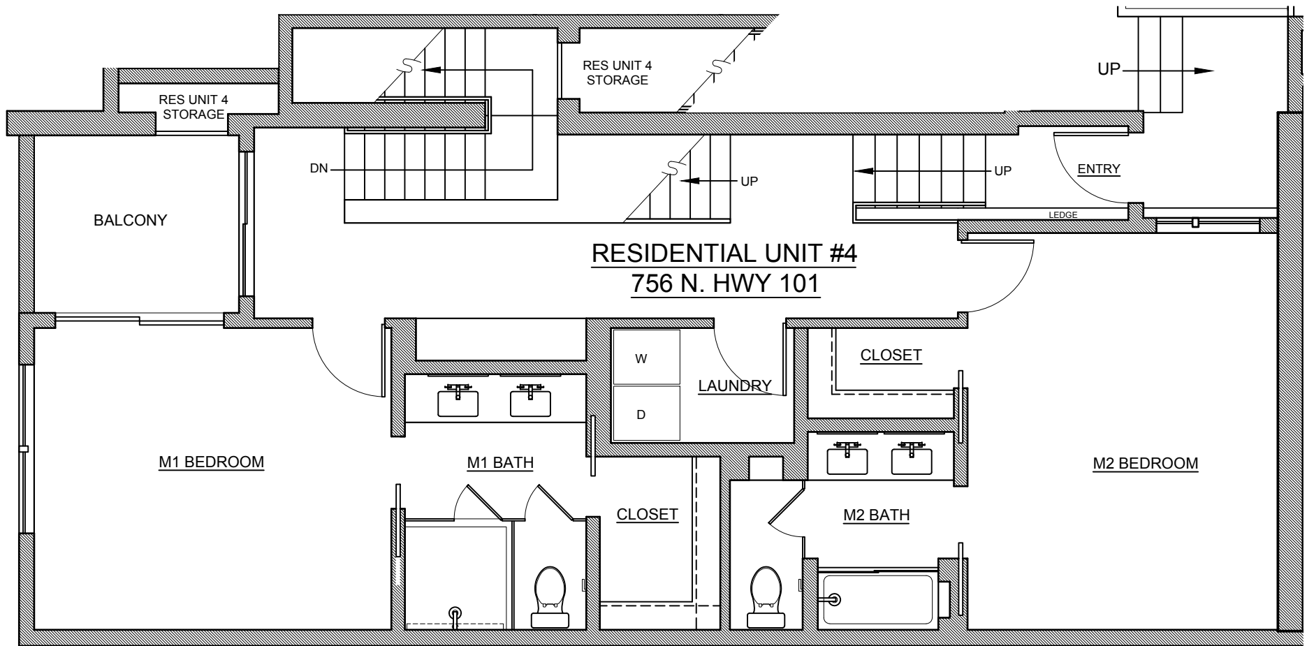
RESIDENCE #4: FIRST FLOOR PLAN
