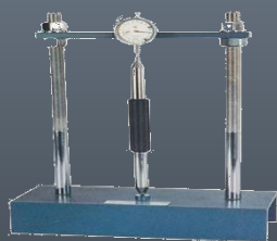
Length Comparator
