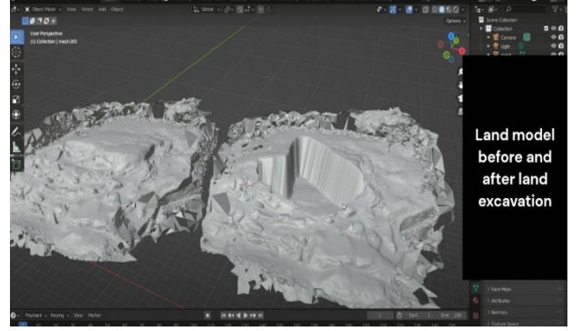
Fig. 7. Generated Model.
