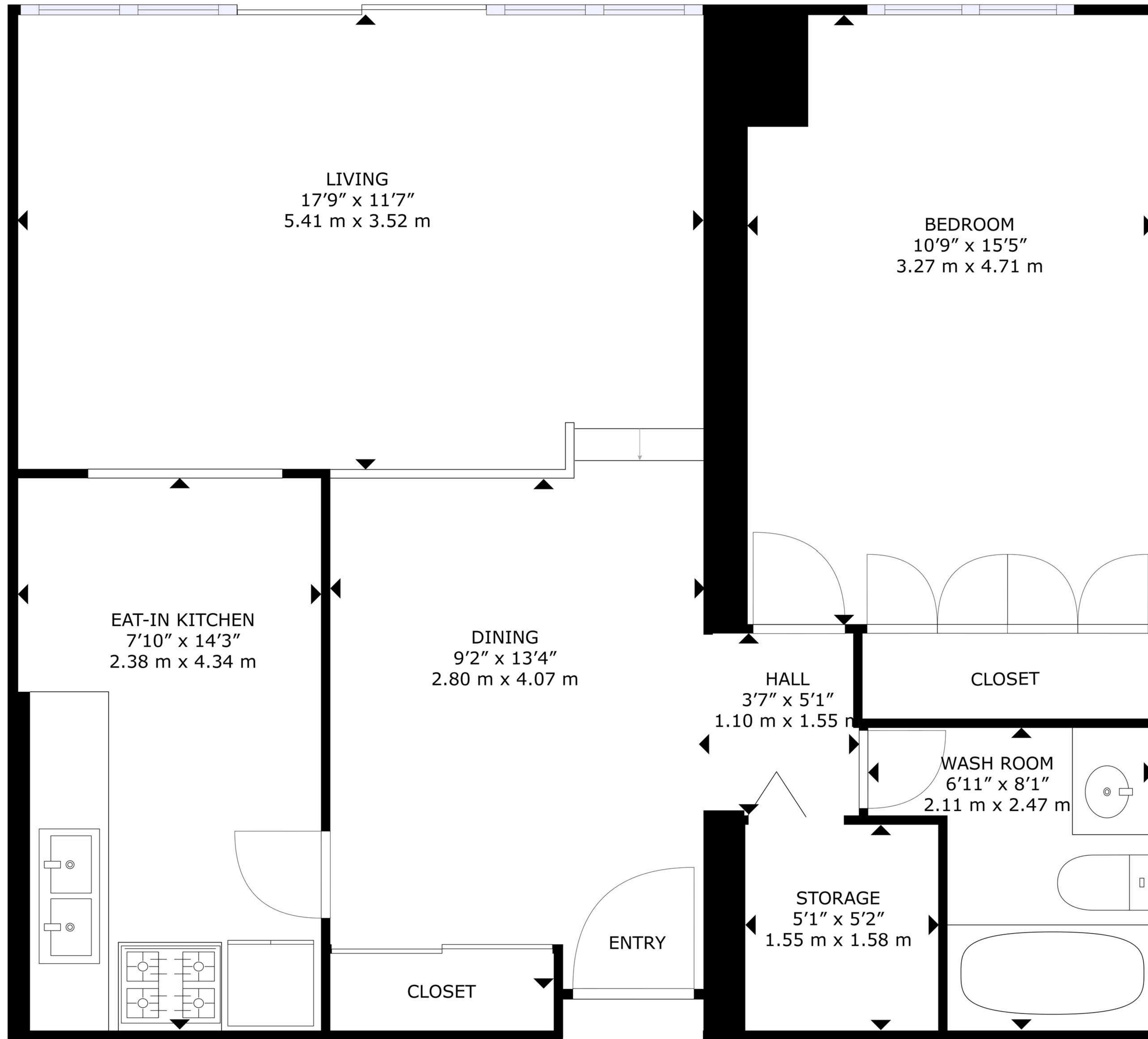
FLOOR PLAN
