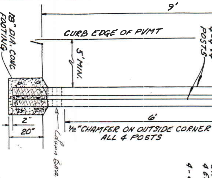
POST SECTION 8 ANCHOR DETAIL
