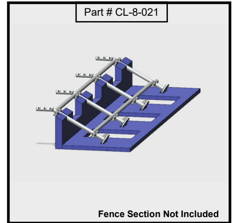
8' Chain-link Security Fence Frame Holding Jig HO Scale (1/87)
