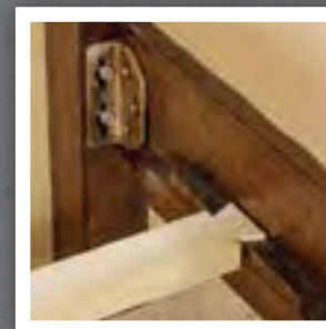
Rail and Slat Dovetail Construction
