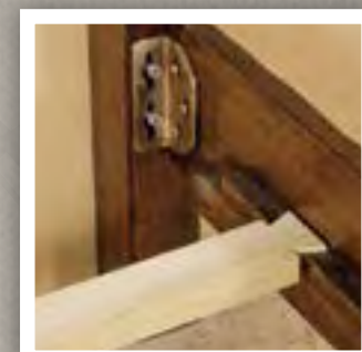
Rail and Slat Dovetail Construction
