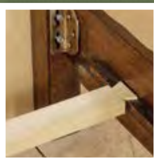
Rail and Slat Dovetail Construction
