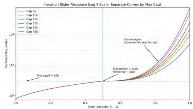
Figure 5 – The iteration slider manual response curve is nonlinear to provide precise control at low iterations.
