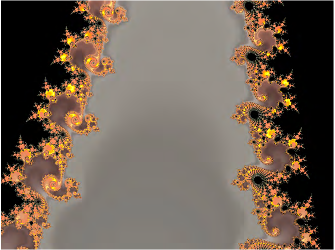
Figure 7 – The Seahorse Valley rendered via Coordinate Jump
