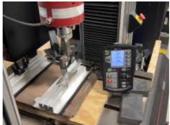
Photo 16: Compression test #2
