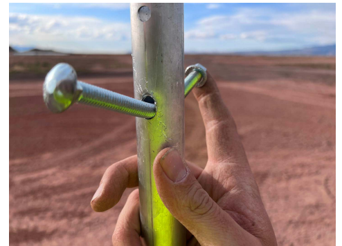
PHOTO 6: First anchor pullout with drilled thru hole deformed
