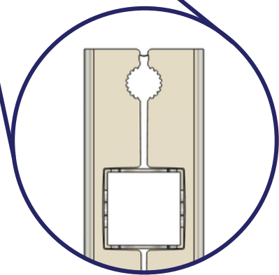
Clamping Teeth
