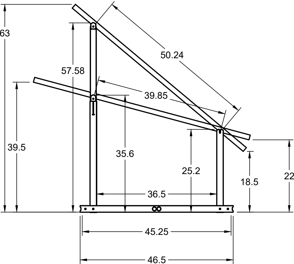
AnchorSpike hole-to-hole dimension: 45.25 inches
