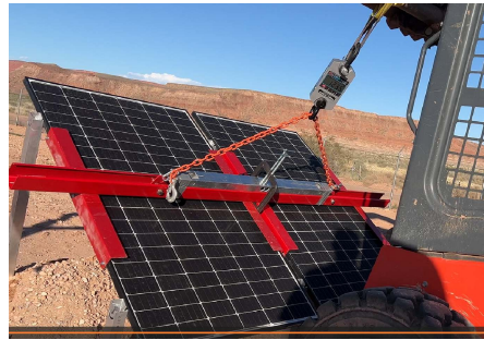
PHOTO 11: Test 2 - Max load
