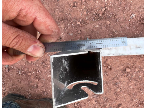
PHOTO 11: Slight deformation after load removed
