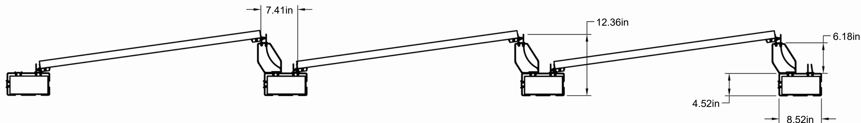
Side View
